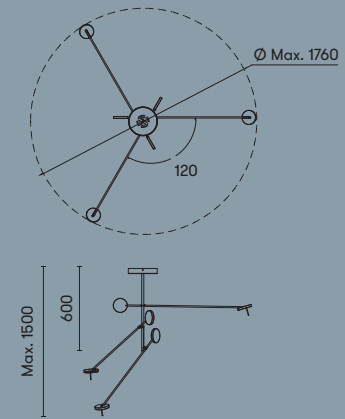
00-5695-05-05 ■ (Standard) 00-5696-05-05 ■ (Mains dimming)*
