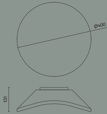
15-5277-BW-M1 (Mains dimming)*
